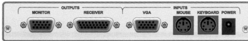
Back Panel Drawing of VGA Extender II Transmitter
